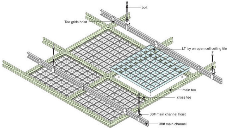
Installation drawing of LT lay on open cell ceiling 595x595mm/595x1195mm
