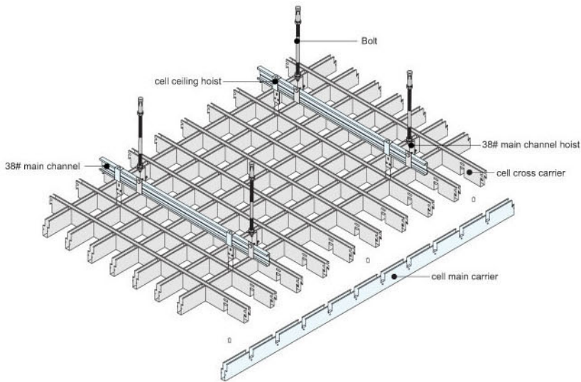
The installation drawing of GA / GB / GC Open cell ceiling
