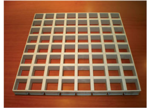
595x595mm lay on open cell ceiling tile with 4 sides trimming (put on tee grids directly) optional spec.:50x50mm/75x75mm/100x100mm/120x120mm/ 150x150mm/200x200mm
