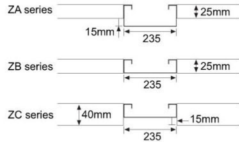
ZA / ZB / ZC TARTAN CEILING PANEL SECTION DRAWING
