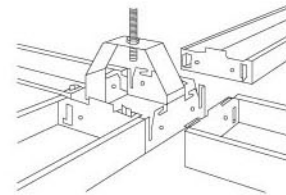
INSTALLATION DRAWING
