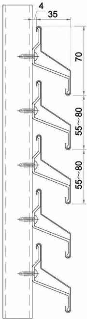
CZ70-SIDE VIEW
